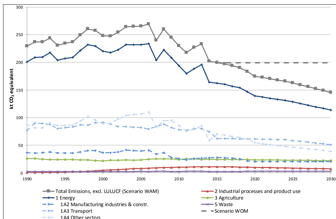
Figure 5-10 Total GHG emissions in CO 2 eq by sector (excl. LULUCF) from 1990 to 2030 for the scenario WAM
