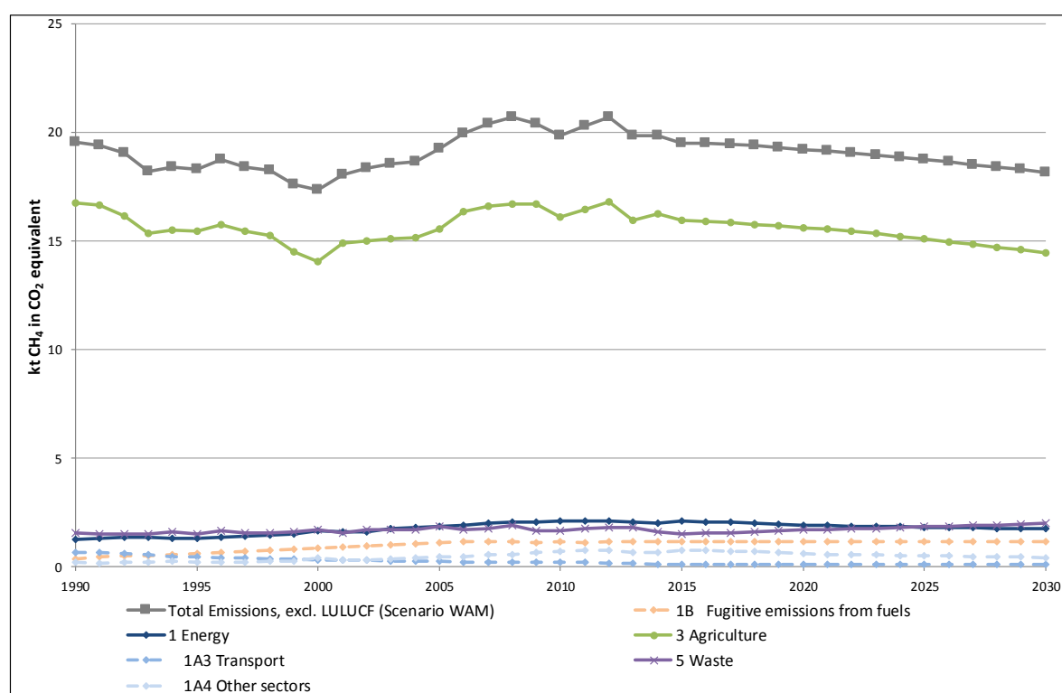
Figure 5-6 CH 4 emissions by sector (excl. LULUCF) from 1990 to 2030 for the scenario WAM
